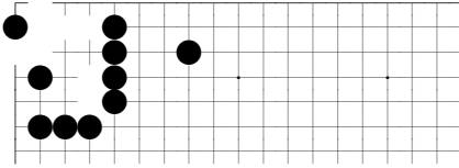
problem 65
