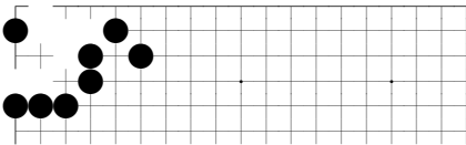
problem 353
