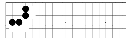
problem 608
