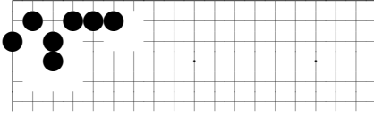
problem 66
