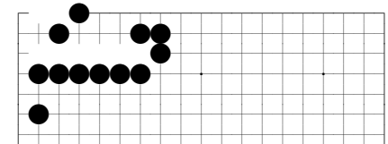
problem 583
