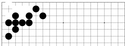
problem 141
