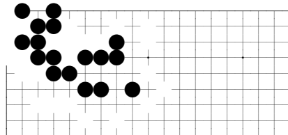
problem 102
