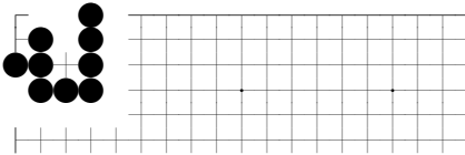
problem 635
