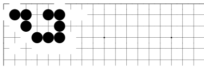
problem 779
