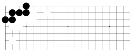
problem 25
