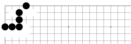
problem 368
