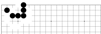
problem 232
