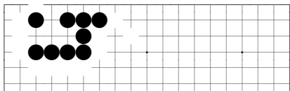
problem 810
