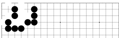
problem 771
