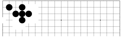
problem 226
