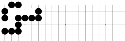
problem 33
