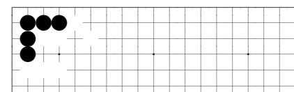
problem 23
