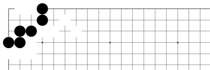
problem 192
