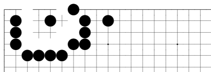
problem 850
