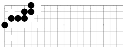
problem 458
