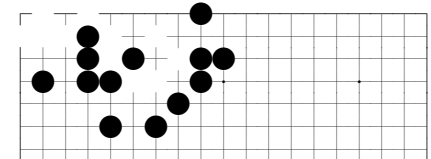
problem 63
