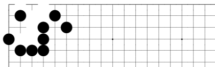
problem 570
