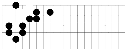
problem 334
