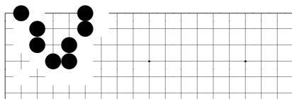
problem 776
