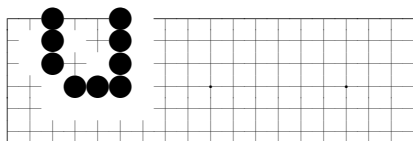
problem 792
