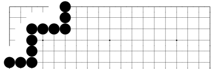
problem 137
