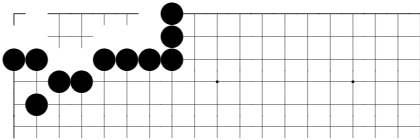
problem 303
