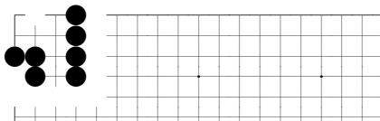
problem 127
