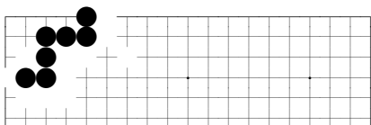
problem 17
