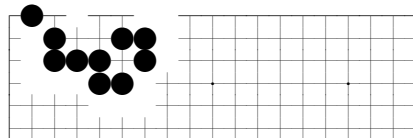
problem 724
