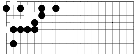
problem 653
