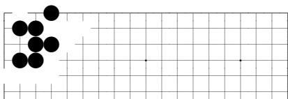
problem 361
