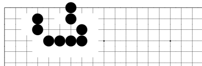
problem 726
