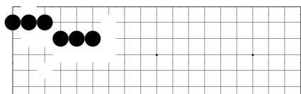
problem 285
