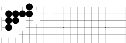
problem 210
