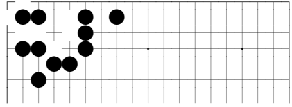
problem 420
