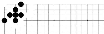
problem 105
