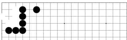
problem 363
