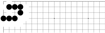
problem 599
