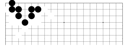
problem 46
