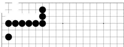
problem 588
