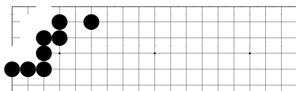
problem 24
