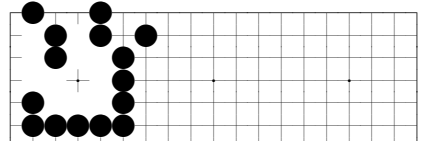
problem 140
