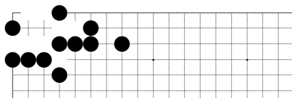
problem 161
