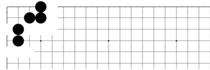
problem 132
