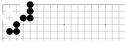
problem 348
