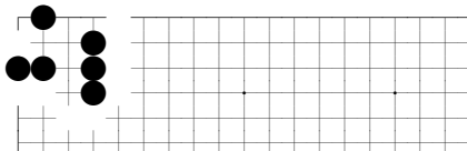
problem 124
