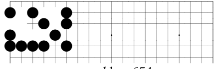
problem 654
