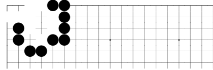
problem 58
